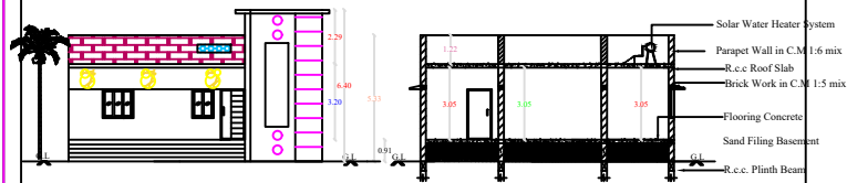
FRONT ELEVATION
