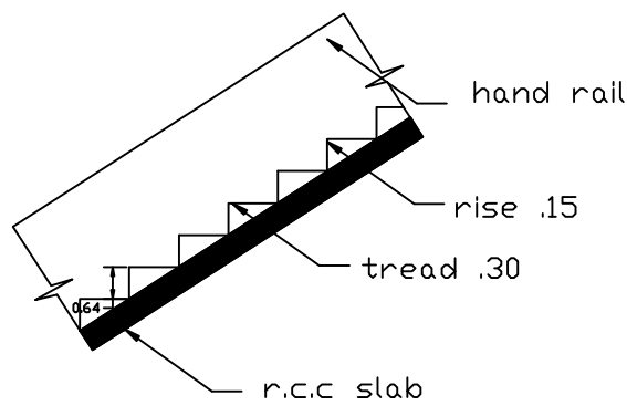
STAIR
