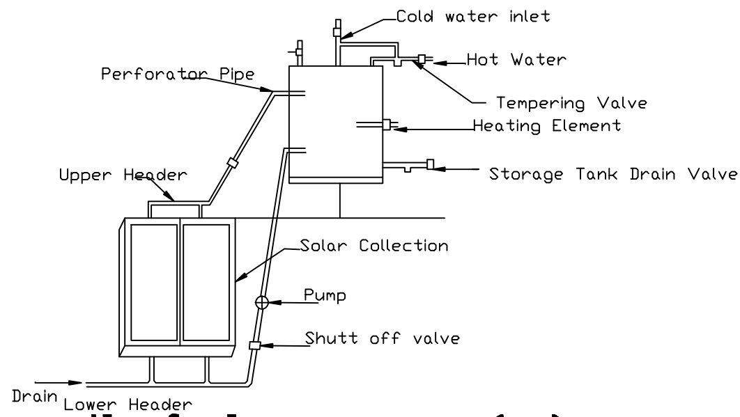
Details of Solar Water Heater (NTS)
