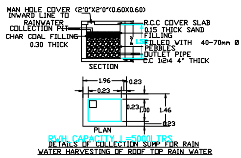
SECTION ON SS
