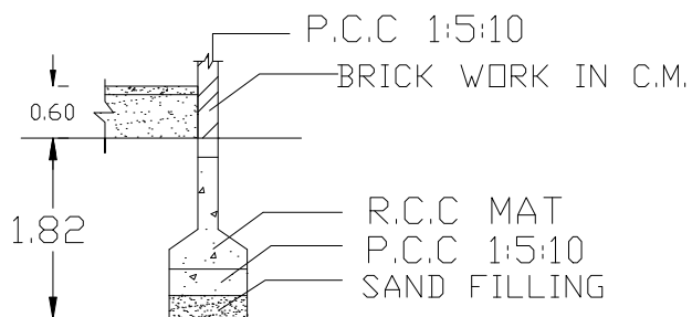
FOUNDATION DETAILS
