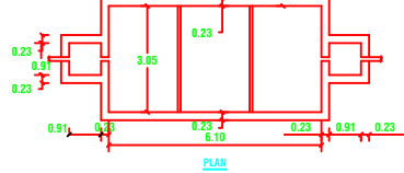
PLAN & SECTION OF SEPTIC TANK & DISPERSION TRENCH
