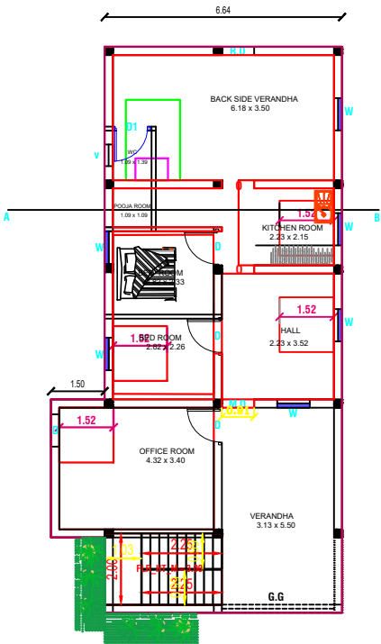
GROUND FLOOR PLAN (WEST FACING)
