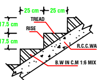
SECTION OF STAIRCASE
