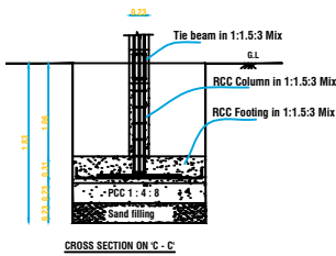
CROSS SECTION ON 'C-C'
