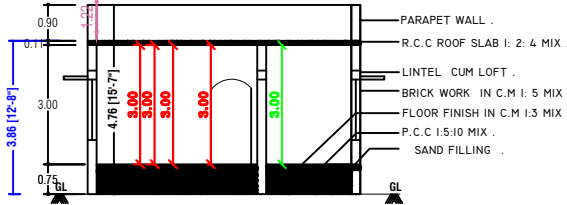
CROSS SECTION ON 'AB'
