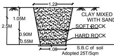
TRIAL PIT DETAILS
