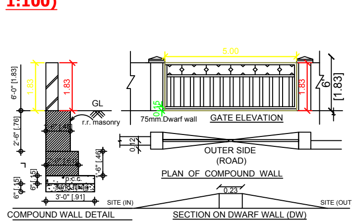
DETAILS OF COMPOUND WALL
