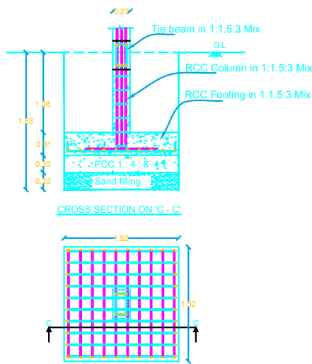
COLOUMN FOUNDATION DETAILS
