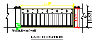
GATE ELEVATION
