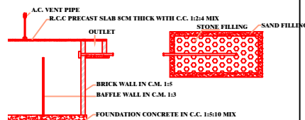
DETAILS OF COLLECTION SUMP FOR RAIN WATER HARVESTING OF ROOF TOP RAIN WATER
