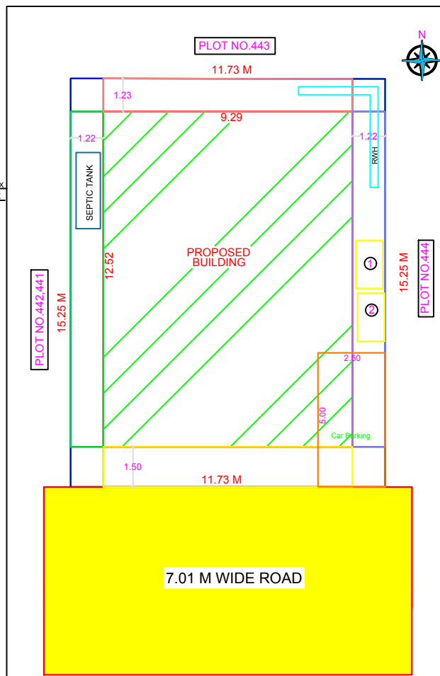
SITE PLAN
