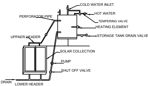
DETAILS OF SOLAR WATER HARVESTING (NTS)
