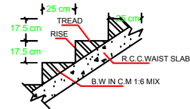
SECTION OF STAIRCASE
