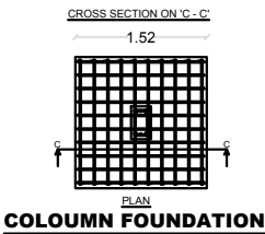
COLOUMN FOUNDATION
