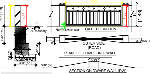
DETAIL OF COMPOUND WALL
