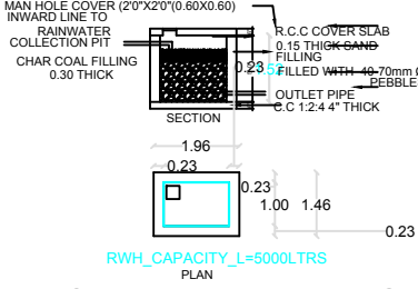
DETAIL OF RAINWATER HARVESTING
