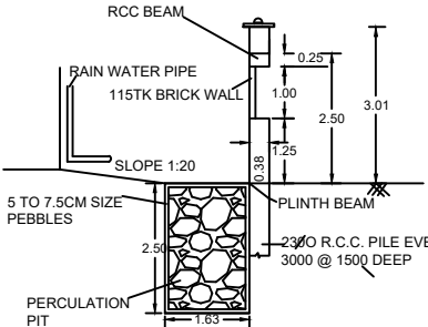
RAINWATER HARVESTING
