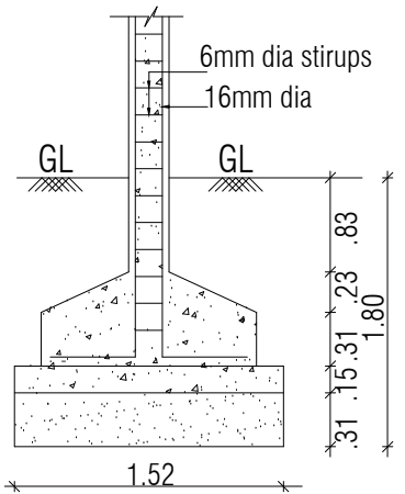
FOUNDATION DETAIL
