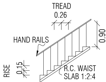
STAIRCASE DETAILS
