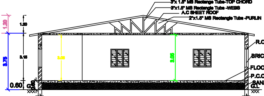
SECTION ON SS
