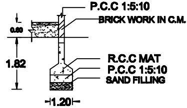
FOUNDATION DETAILS
