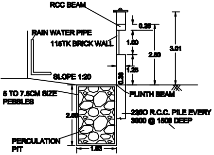
RAINWATER HARVESTING
