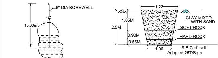
TRIAL PIT DETAILS
