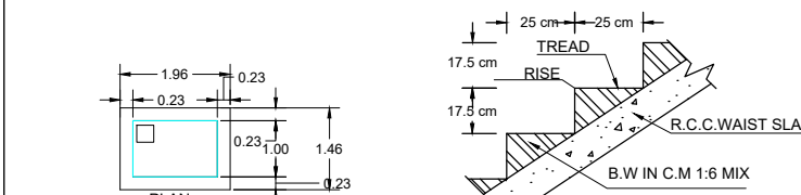
SECTION OF STAIRCASE
