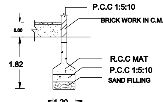
FOUNDATION DETAILS
