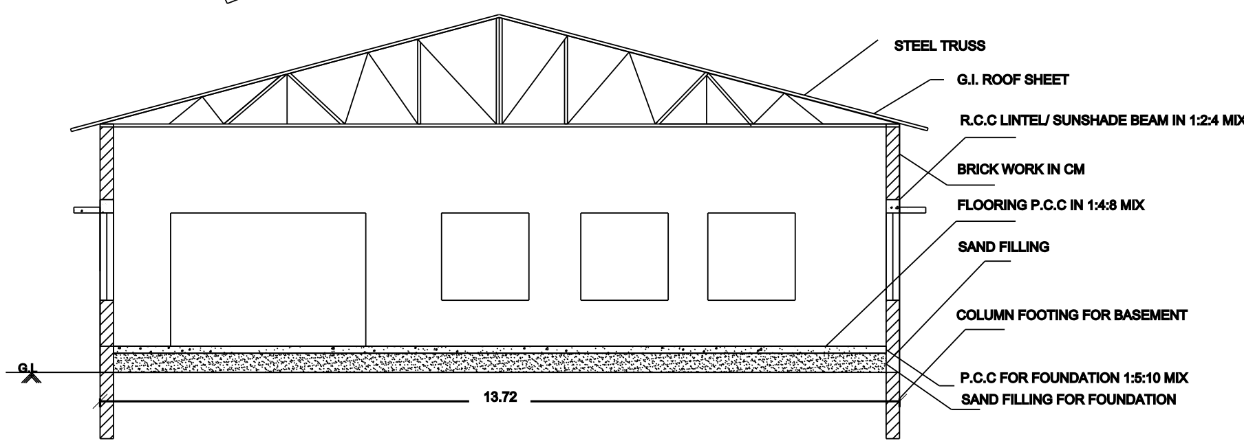
SECTION ON-AA
