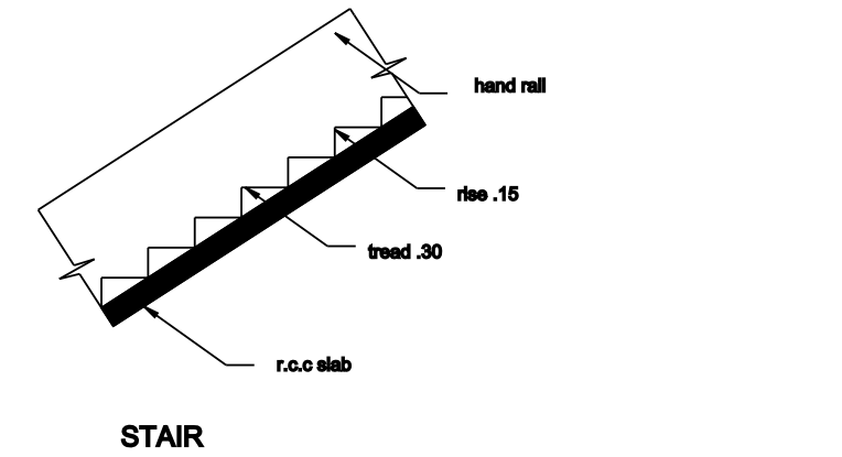
STAIR
