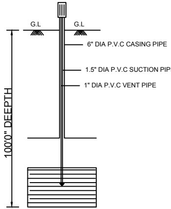
BORE WELL
