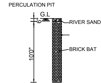
PERCOLATION PIT
