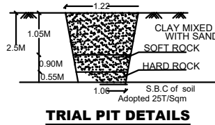
TRIAL PIT DETAILS
