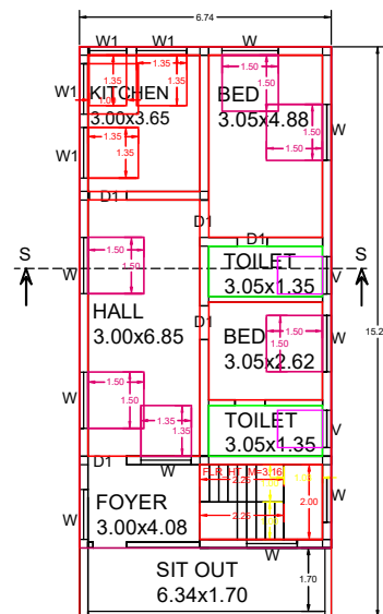
PROPOSED FIRST FLOOR
