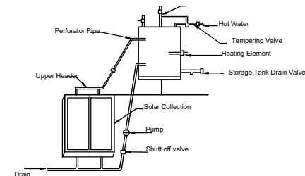
Details of Solar Water Heater (NTS)
