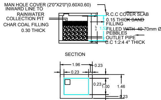
RWH_CAPACITY_L=5000LTRS
