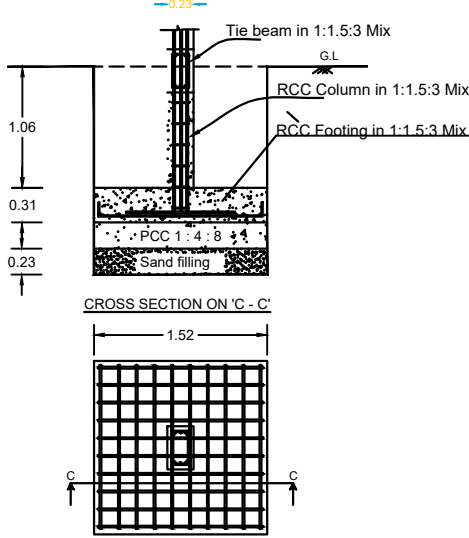
COLOUMN FOUNDATION
