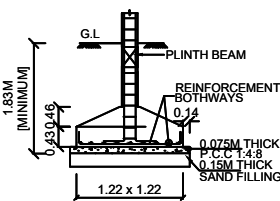
COLUMN FOOTING ( REFER STRUCTURAL DRAWING )
