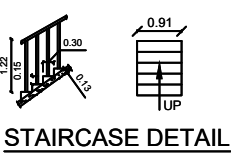
STAIRCASE DETAIL
