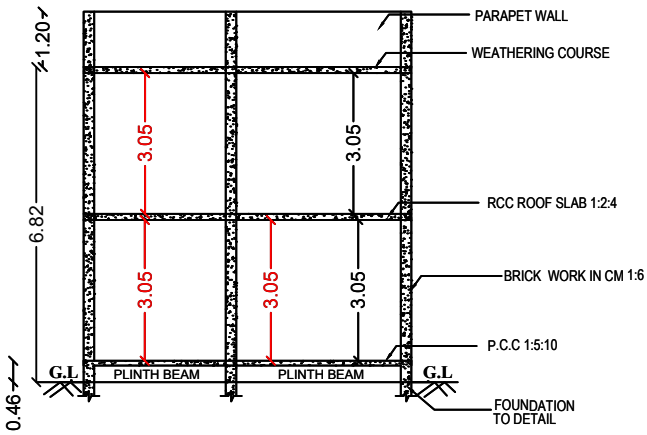
SECTION ON "A-L"
