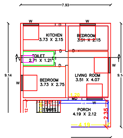
FLOOR PLAN
