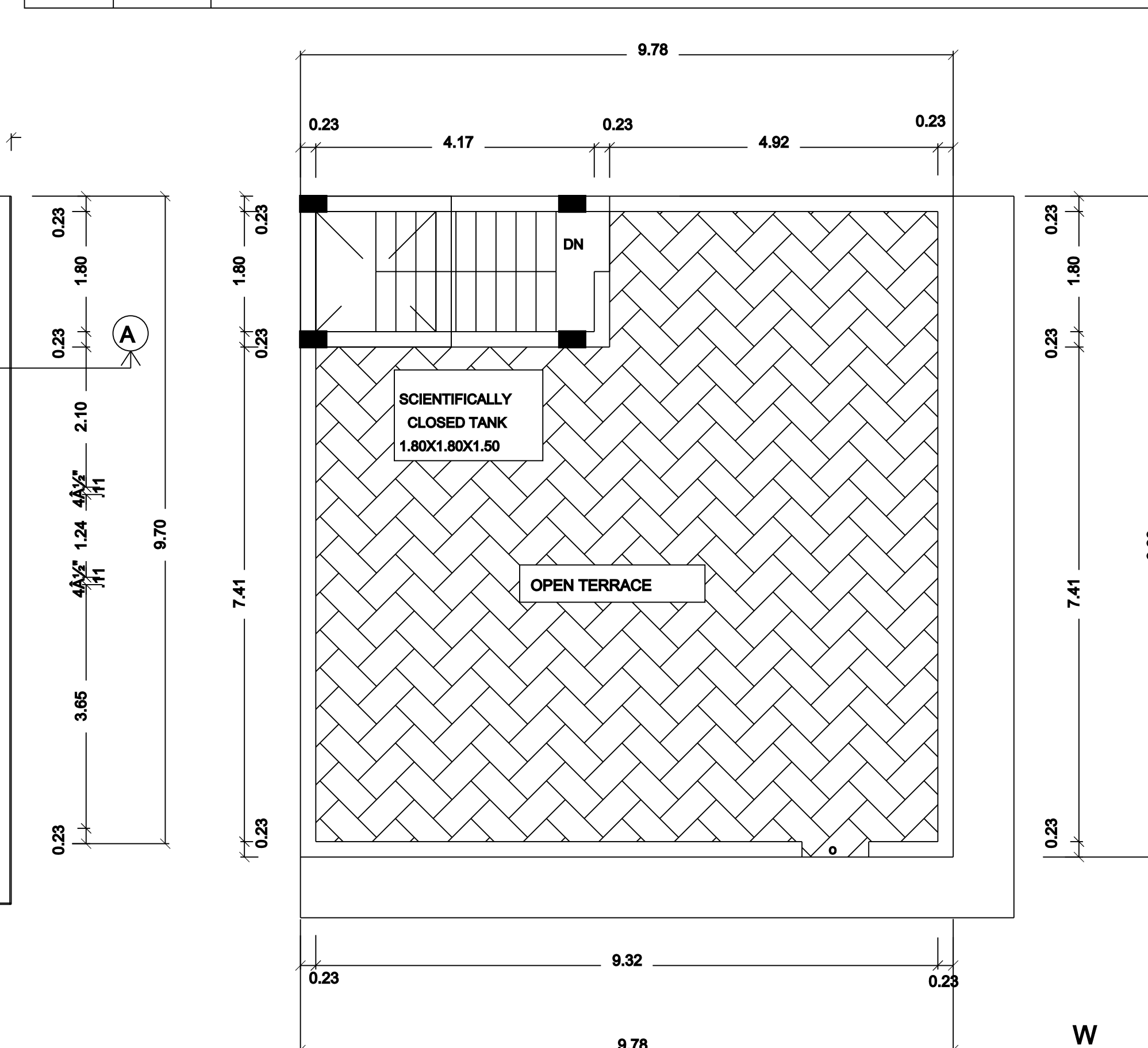
TERRACE_FLOOR_PLAN
