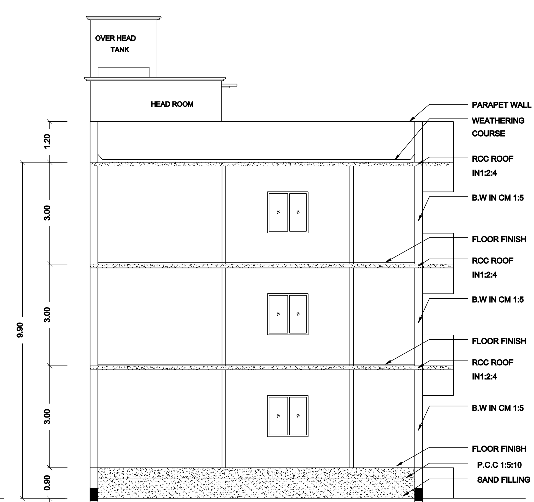
SECTION AA'
