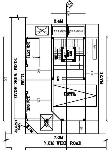
SITE CUM STILL FLOOR PLAN (PROPOSED)
