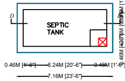
PLAN OF SEPTIC TANK SCALE 1"=2'-0"
