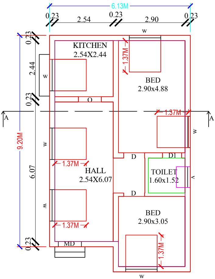
FLOOR PLAN
