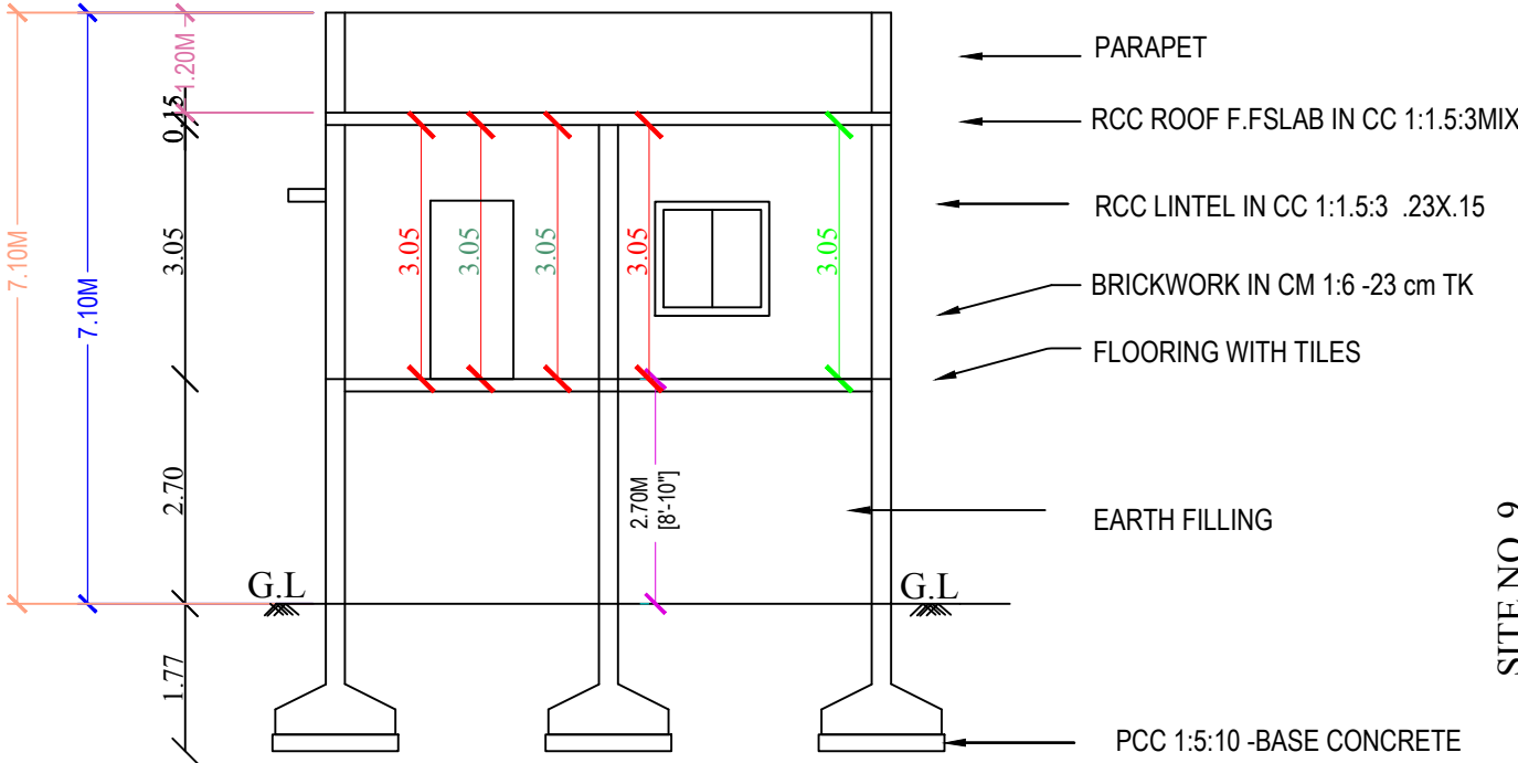
SECTION AA
