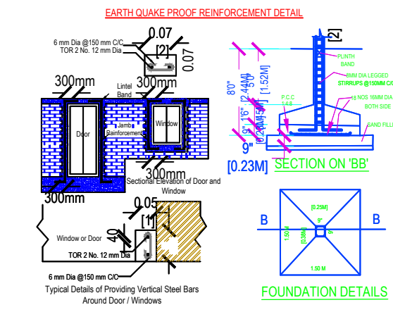
FOUNDATION DETAILS
