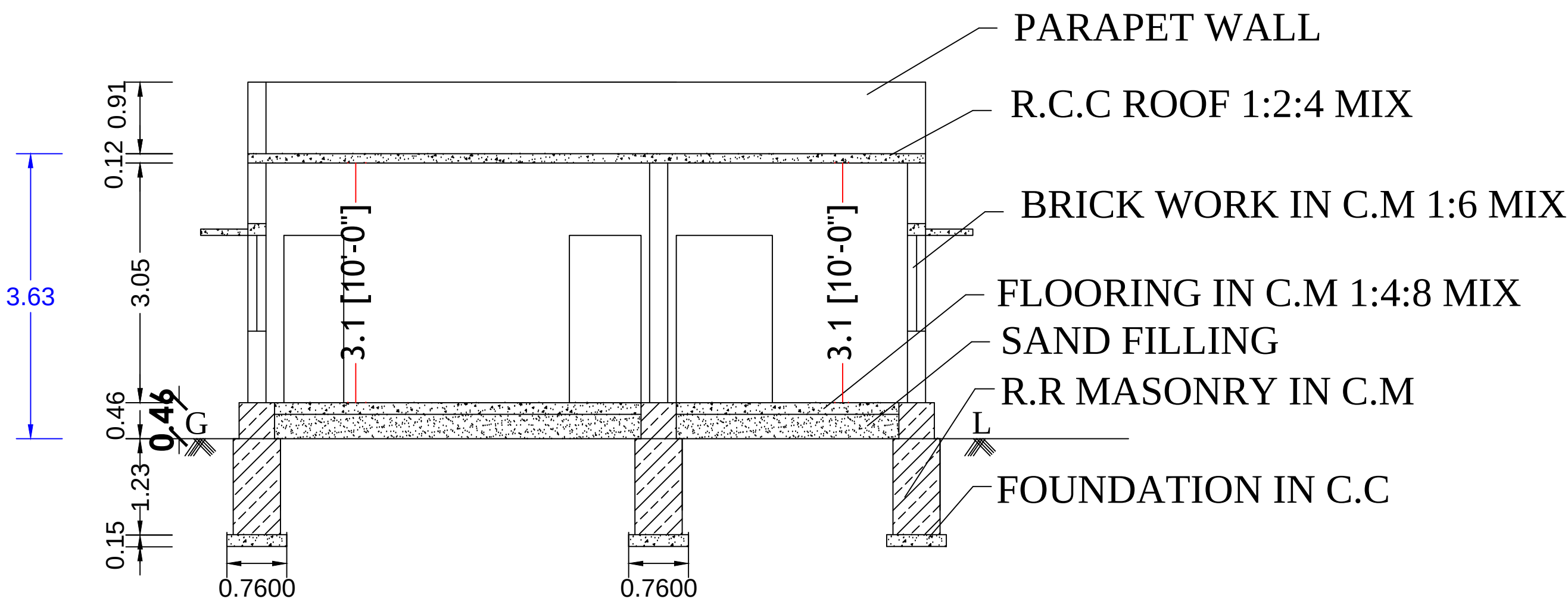
SECTION AA'
