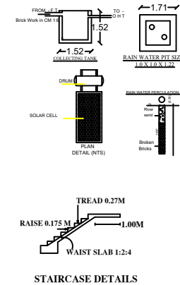
STAIRCASE DETAILS
