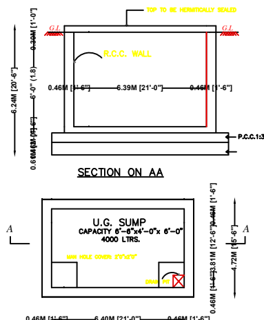
SUMP DETAIL SCALE 1"=4'0"
