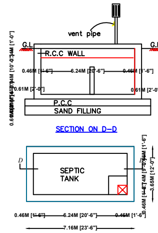
PLAN OF SEPTIC TANK SCALE 1"=2'0"
