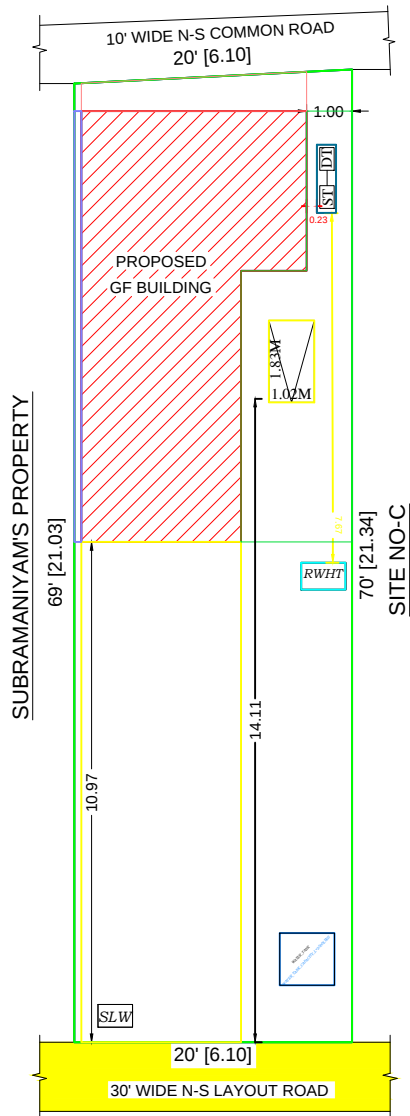
SITE PLAN
