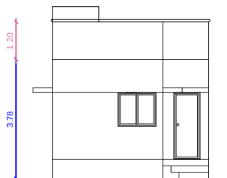
ELEVATION-B
