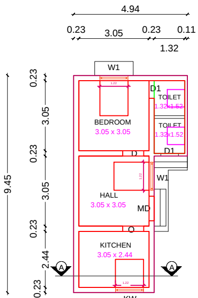
PRO.GROUND FLOOR PLAN
