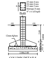
COLUMN DETAILS
