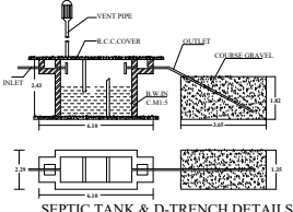
SEPTIC TANK & D-TRENCH DETAILS
