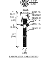
RAIN WATER HARVESTING PERCOLATION PIT
