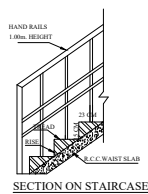
SECTION ON STAIRCASE
