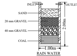
RAIN WATER COLLECTION TANK
