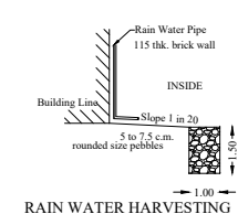
RAIN WATER HARVESTING
