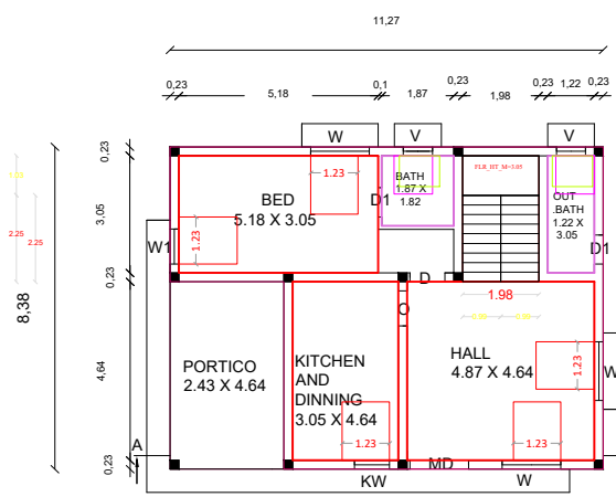
GROUND FLOOR PLAN FACING EAST
