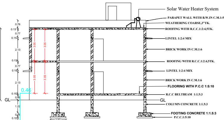
SECTION FACING ON A&A'
