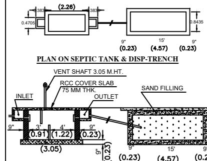
SECTION ON SEPTIC TANK & DISP-TRENCH
