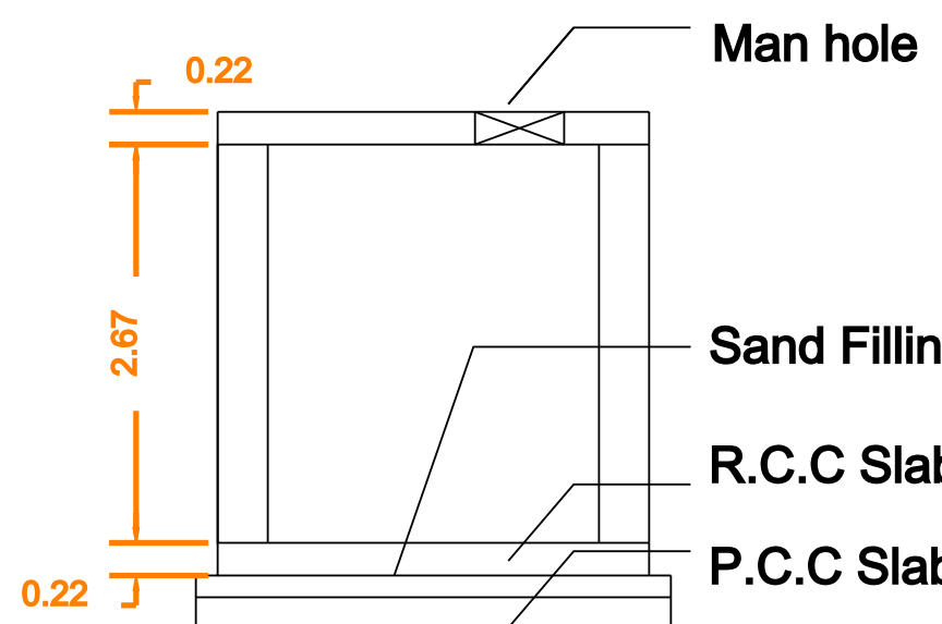
SUMP DETAILS
