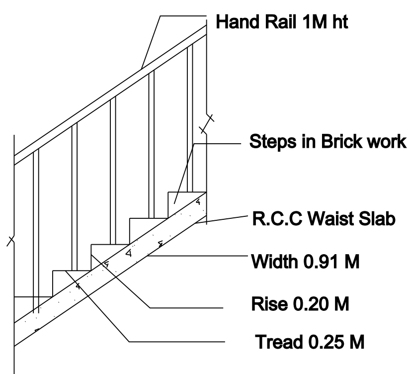
STAIRCASE DETAILS
