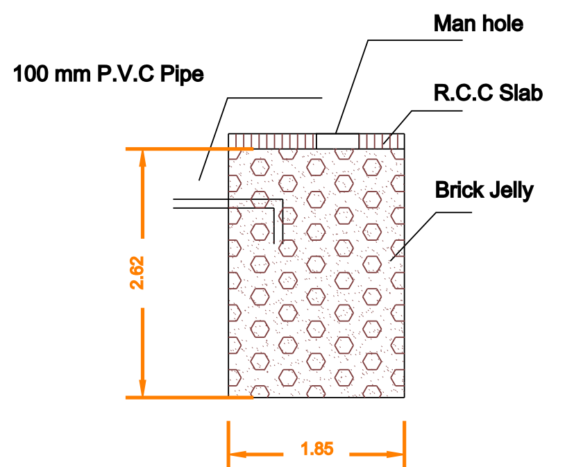
SECTION OF RAINWATER COLLECTION TANK
