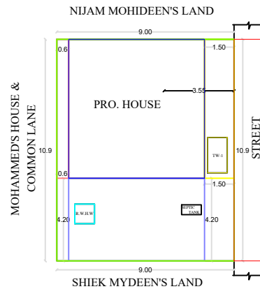
SITE PLAN
