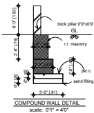
COMPOUND WALL DETAIL SCALE: 1/1" = 4'-0"
