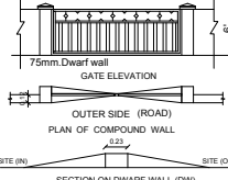
OUTER SIDE (ROAD) PLAN OF COMPOUND WALL SCALE: 1/1" = 4'-0"
