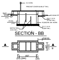
SECTION - BB PLAN OF SEPTIC TANK
