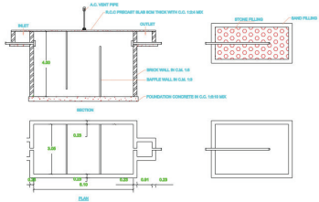
SECTION OF SEPTIC TANK & DISPERSION TRENCH
