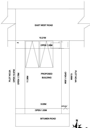
SITE PLAN
