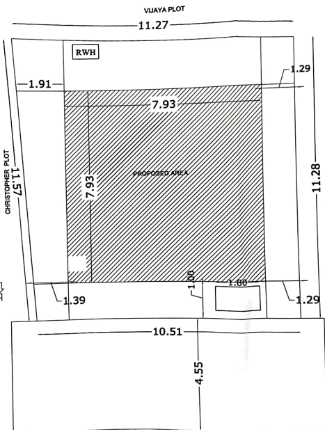
SITE PLAN
