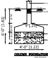
COLUMN FOUNDATION (NOT TO SCALE)
