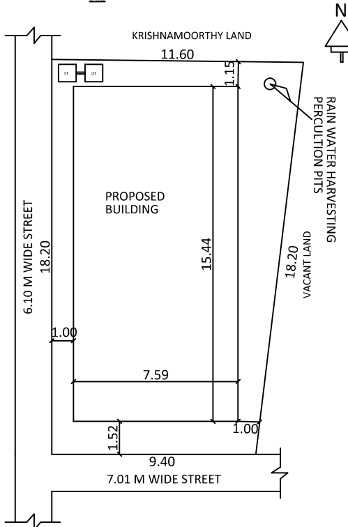
SITE PLAN
