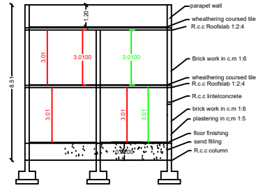
SECTION ON XX
