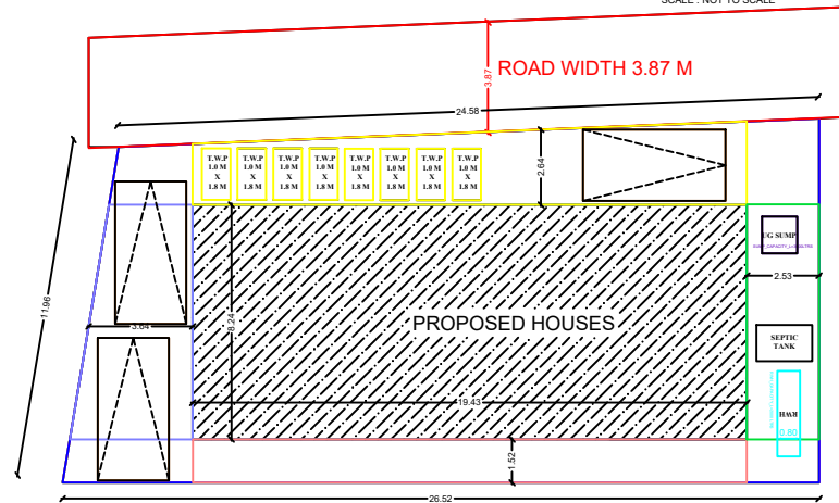
SITE PLAN
