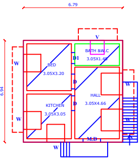
EXG-HOUSE PLAN DOOR NO:21
