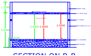
SECTION ON 'BB'
