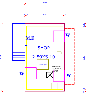
SHOP PLAN PROPOSED GROUND FLOOR PLAN
