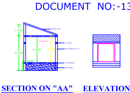
SECTION ON "AA" ELEVATION
