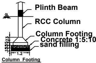
Foundation Detail
