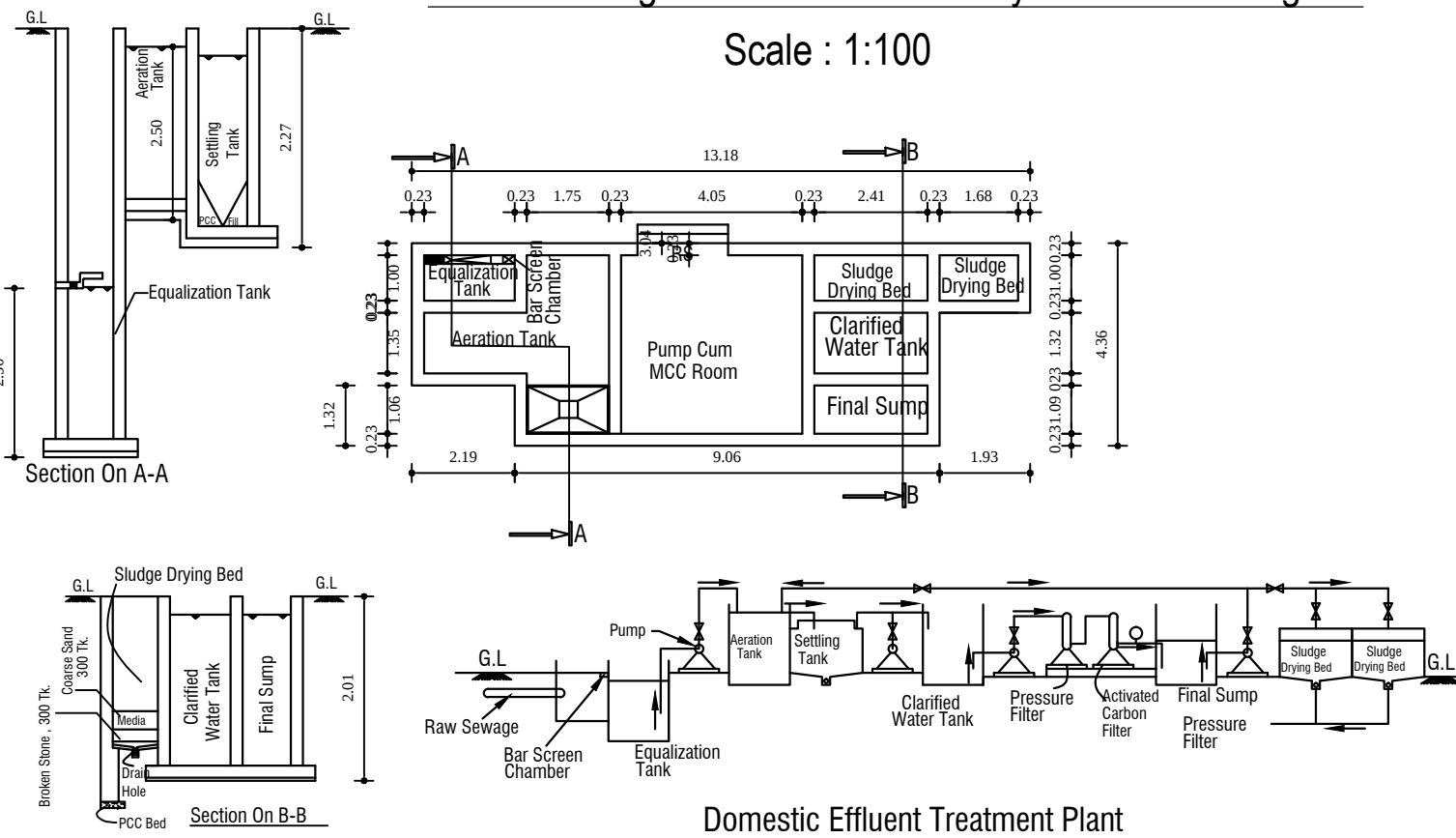
Domestic Effluent Treatment Plant Hydraulic Flow Diagram
