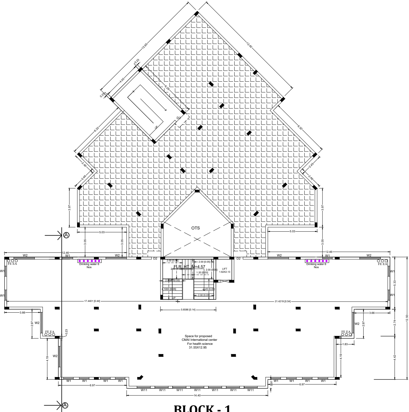
BLOCK - 1 THIRD FLOOR PLAN
