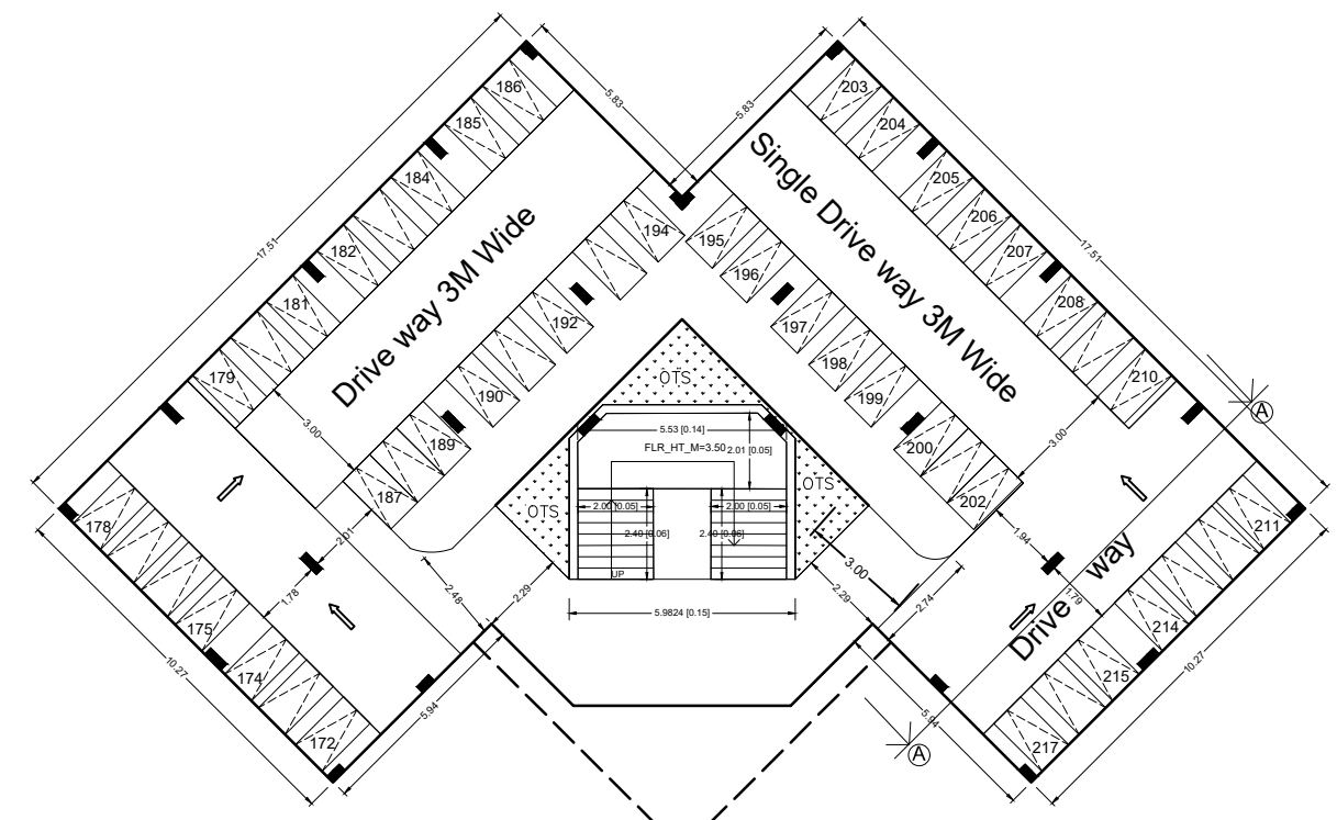
BLOCK - 2 STILT FLOOR PLAN
