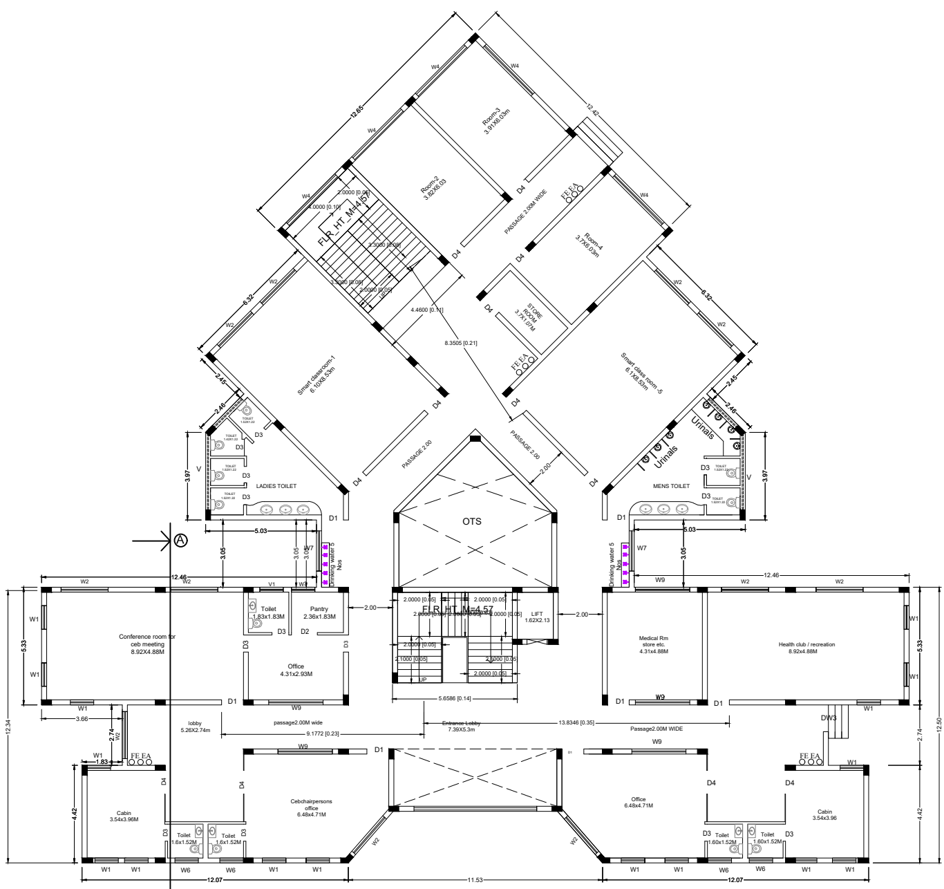
BLOCK - 1 FIRST FLOOR PLAN
