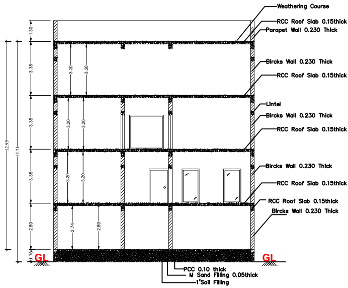
BLOCK - 1 SECTION A-A
