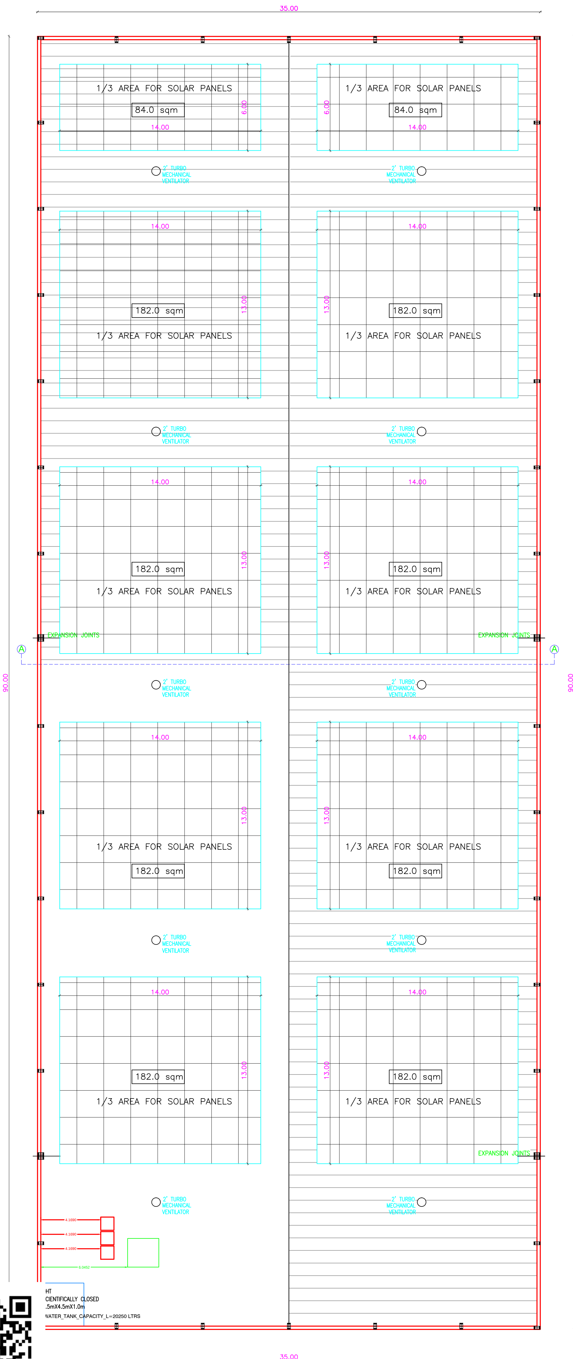
ROOF PLAN
