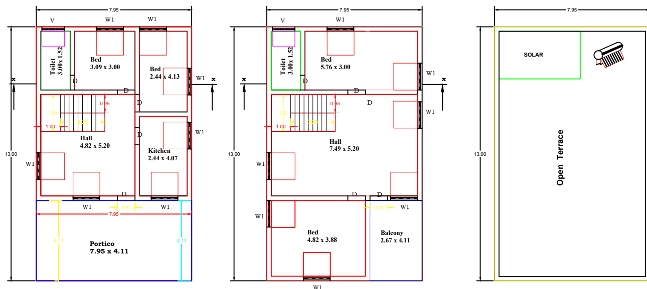
Proposed Terrace Floor Plan
