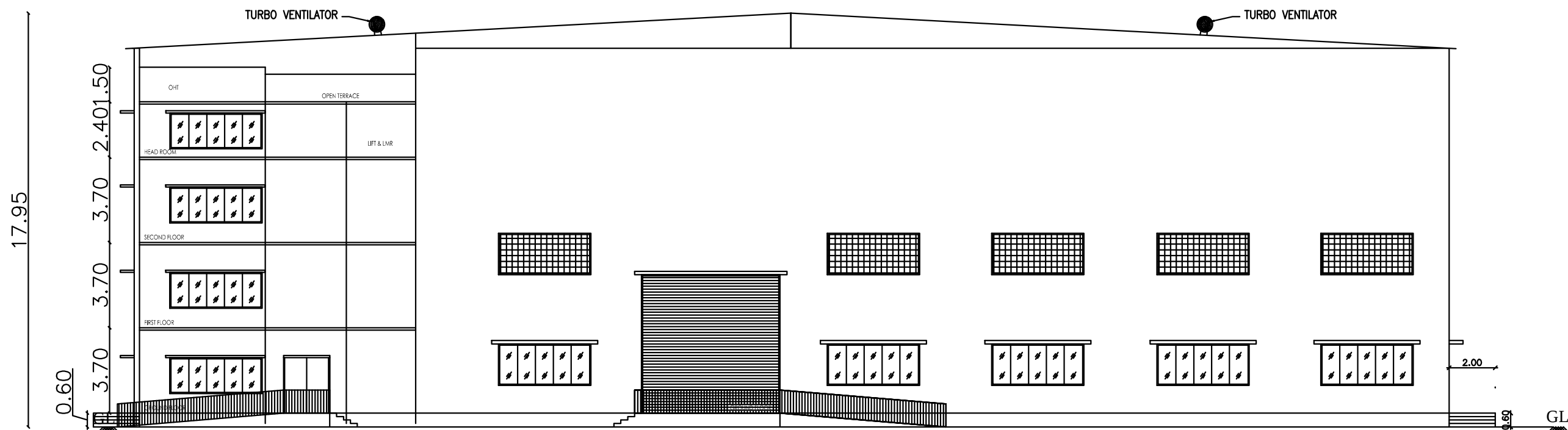
SOUTH FACING ELEVATION
