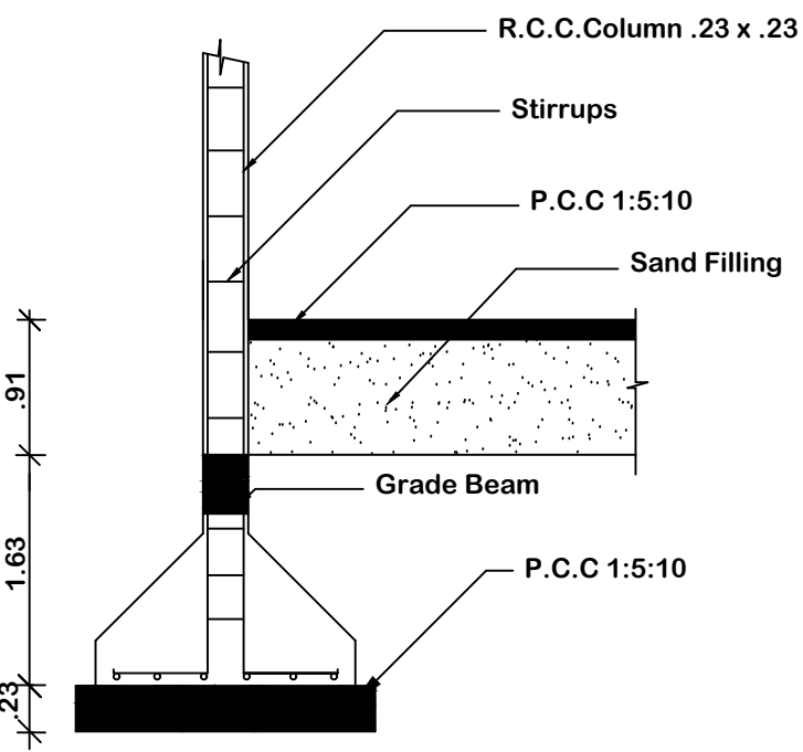
COLUMN DETAIL
