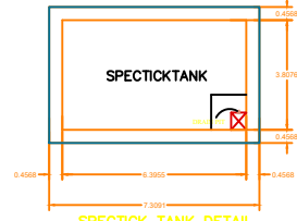
SPECTICK TANK DETAIL SCALE 1"=40"
