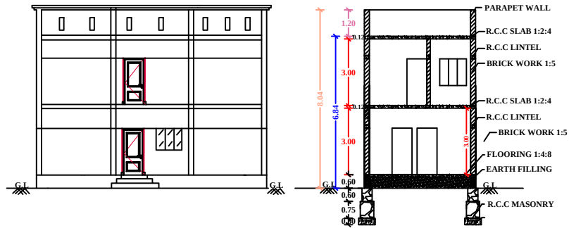
FRONT ELEVATION
