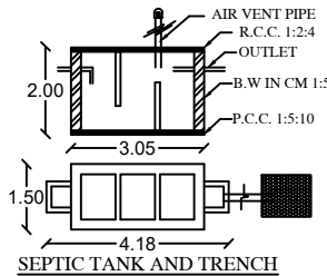
SEPTIC TANK AND TRENCH
