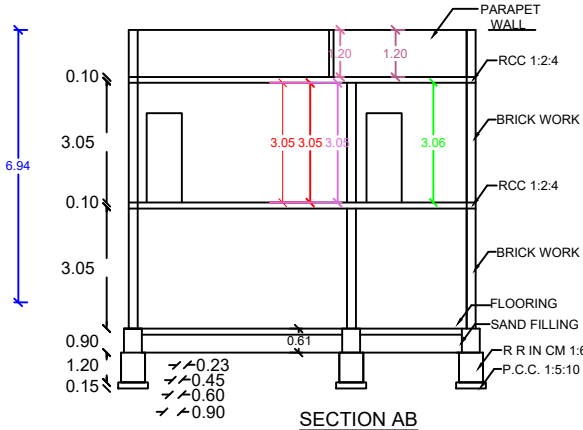
SECTION AB
