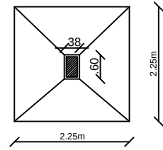
PLAN TYPICAL SECTION OF FOOTING
