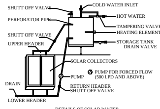
DETAILS OF SOLAR WATER HEATING SYSTEM
