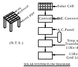
SOLAR SYSTEM FLOW DIAGRAM
