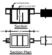
Section Plan Septic Tank & Trench
