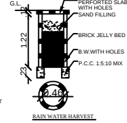
RAIN WATER HARVEST
