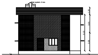
FRONT ELEVATION
